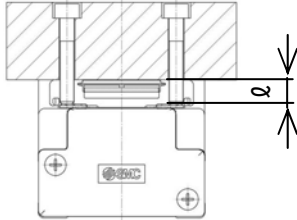
Work piece mounting
